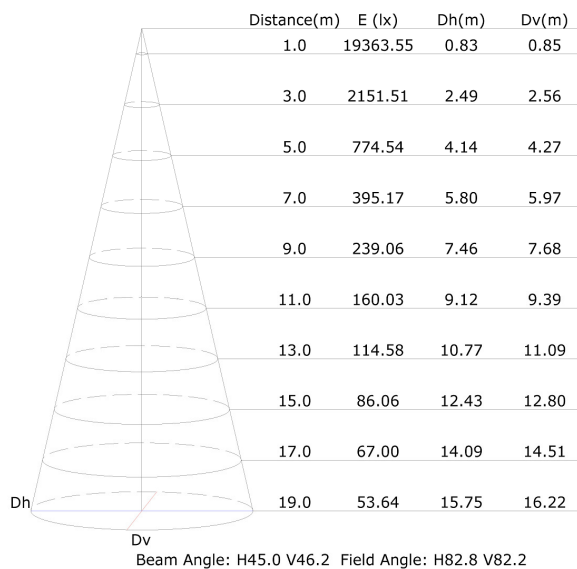
Illuminance at a Distance
